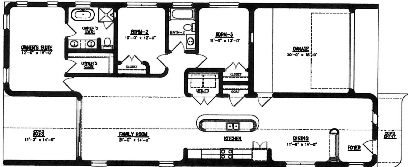
FLOOR PLAN
